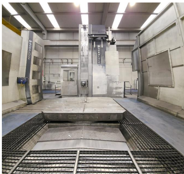
Mesa rototraslante DEMMELER DRLTS2500 3000x2500 mm. Rototranslating table DEMMELER mod. DRLTS2500. 3000 X 2500 mm
